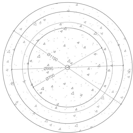
Plan Elevation
